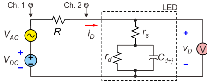
Figure 3 The circuit for measuring the dynamic response of an LED. In the dashed rectangle is an equivalent circuit of the measured LED.
