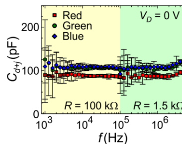
Figure 6 The frequency-dependent capacitance characteristics of three LEDs in low frequency (1 kHz to 100 kHz) and high frequency (100 kHz to 5 MHz) ranges. A constant V_{DC} of 0 V is applied during the measurement.
