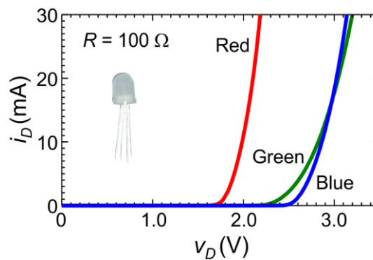
Figure 2 The I - V characteristics of three LEDs in an RGB-LED package.
