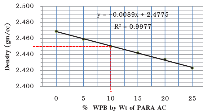
Figure 3 Density values and quantity of plastic bag waste added to the para-asphalt concrete
