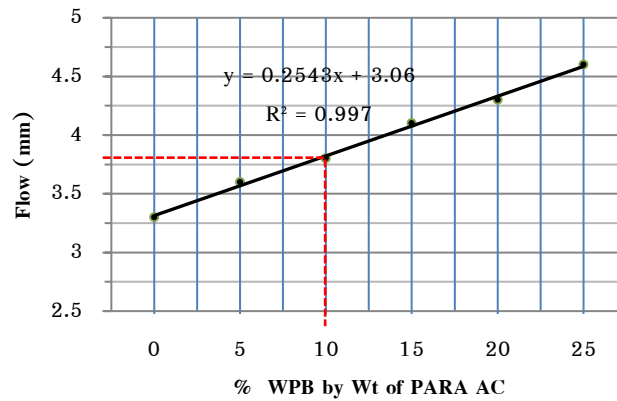
Figure 6 Flow values and quantity of plastic bag waste added to the para-asphalt concrete
