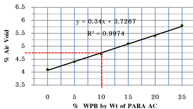
Figure 4 Air void values and quantity of plastic bag waste added to the para-asphalt concrete
