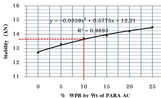
Figure 5 The Marshall stability values and quantity of plastic bag waste added to the para-asphalt concrete
