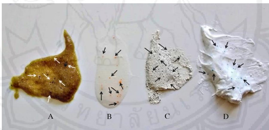
Figure 1 Primary microplastics (arrows) in skin care products and toothpaste A and C = body cleansing, B = facial cleansing and D = toothpaste
