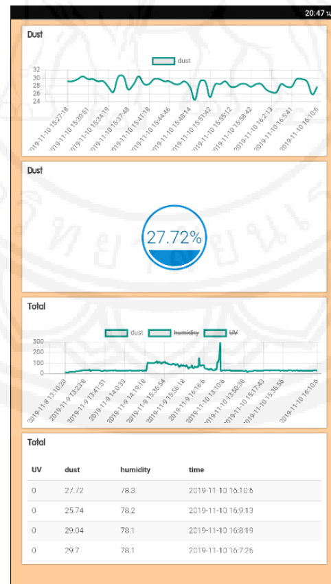
Figure 20 Web Dashboard
