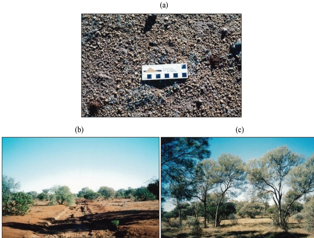
Figure 12: Regolith materials and landscape view for the ACap regolith -landform unit; (a) sand, silt and quartz gravel; (b) channel deposit and (c) high Acacia aneura tree with a common of understory bush, Eremophila forrestii , and Eremophila fraseri , Meekatharra, Western Australia.
