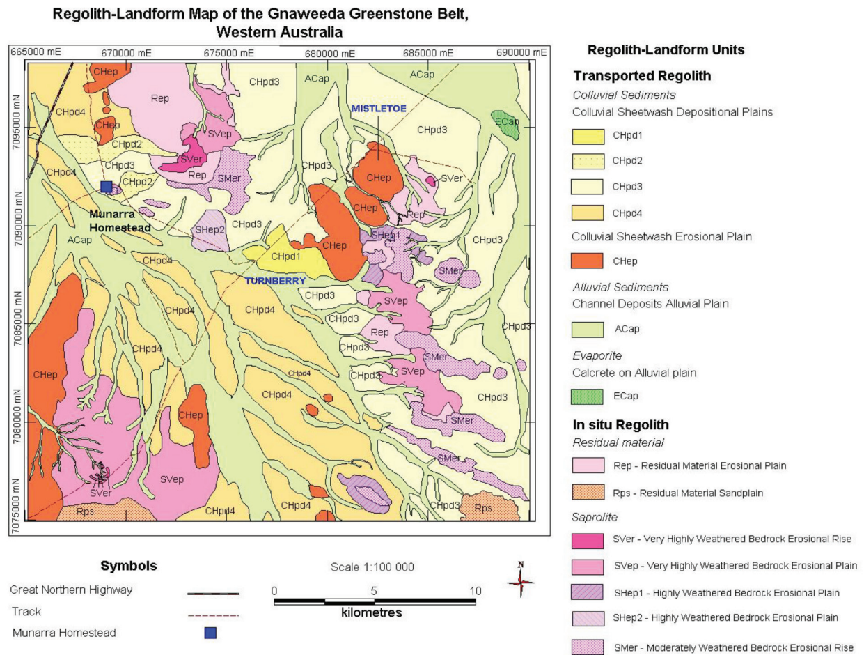
Figure 7: Regolith-landform map of the Gnaweeda Greenstone Belt, Western Australia (UTM GDA94, MGA Zone 50).
